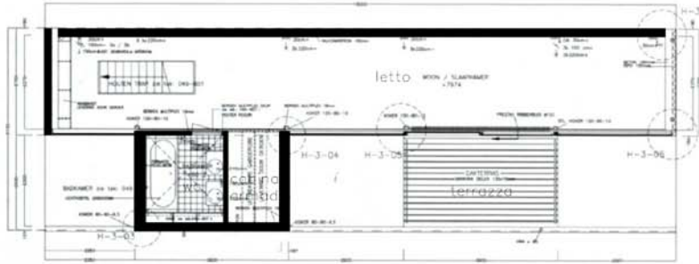
Pianta tercera / Third floor plan
