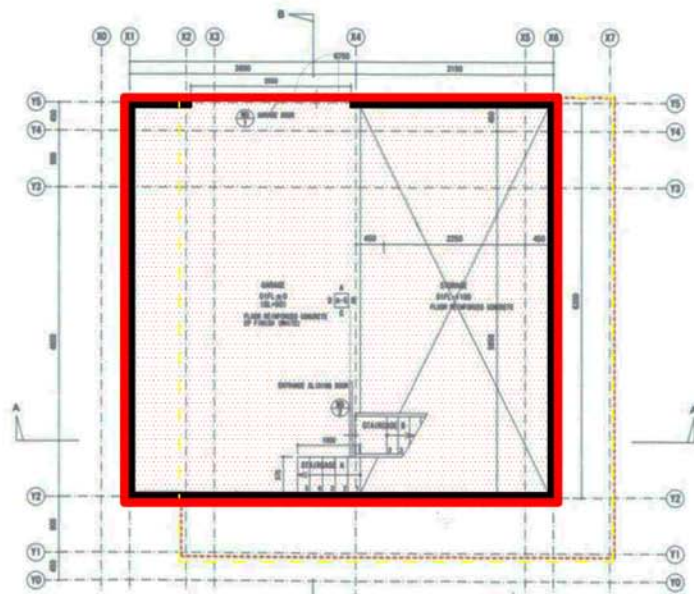
Planta baja / Ground floor plan
