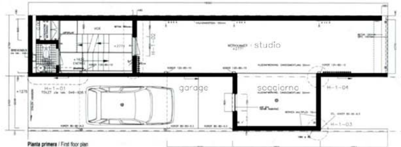
Pianta primera / First floor plan
