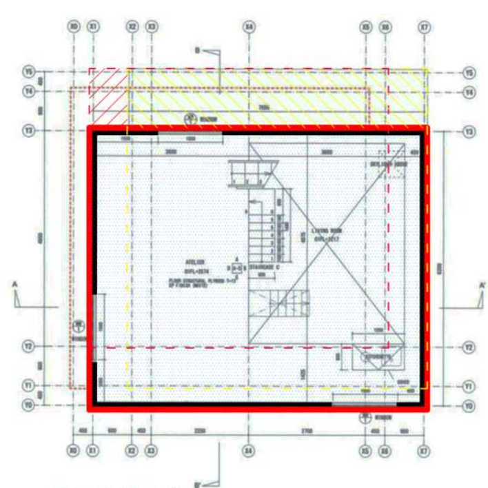
Planta segunda / Second floor plan
