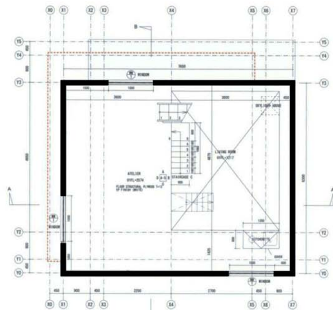
Planta segunda / Second floor plan
