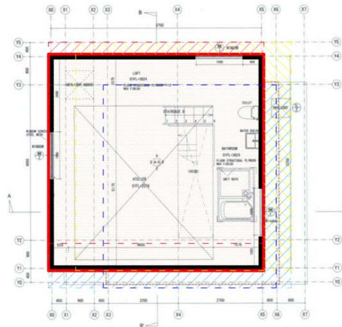
Planta tercera / Third floor plan
