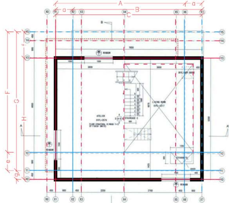
Planta segunda / Second floor plan
