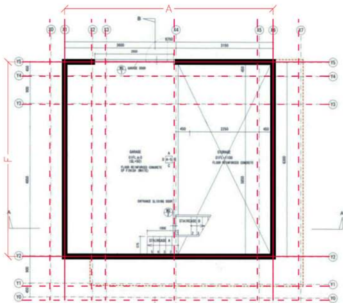
Planta baja / Ground floor plan
